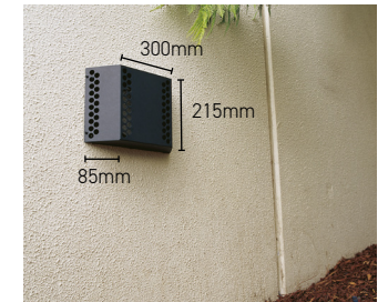
Flue cowl attached to external wall with Chateau installed into stud wall cavity
